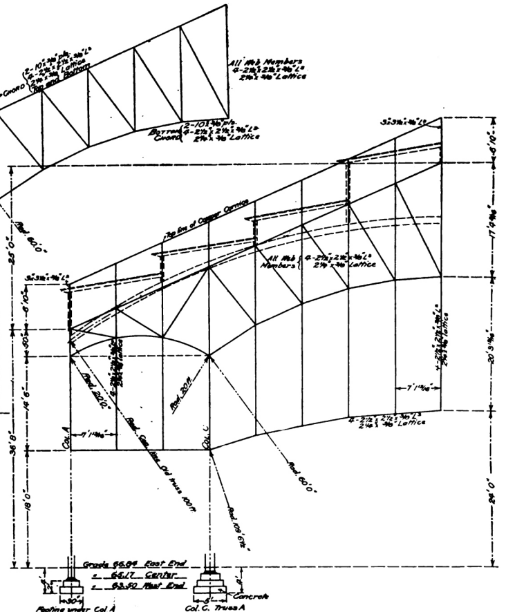
Fig. 4.—One-half Elevation of End Truss, Union Station, Columbus, O.
