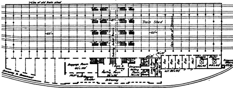
Fig. 1.—Plan of Basement (Track Level).
